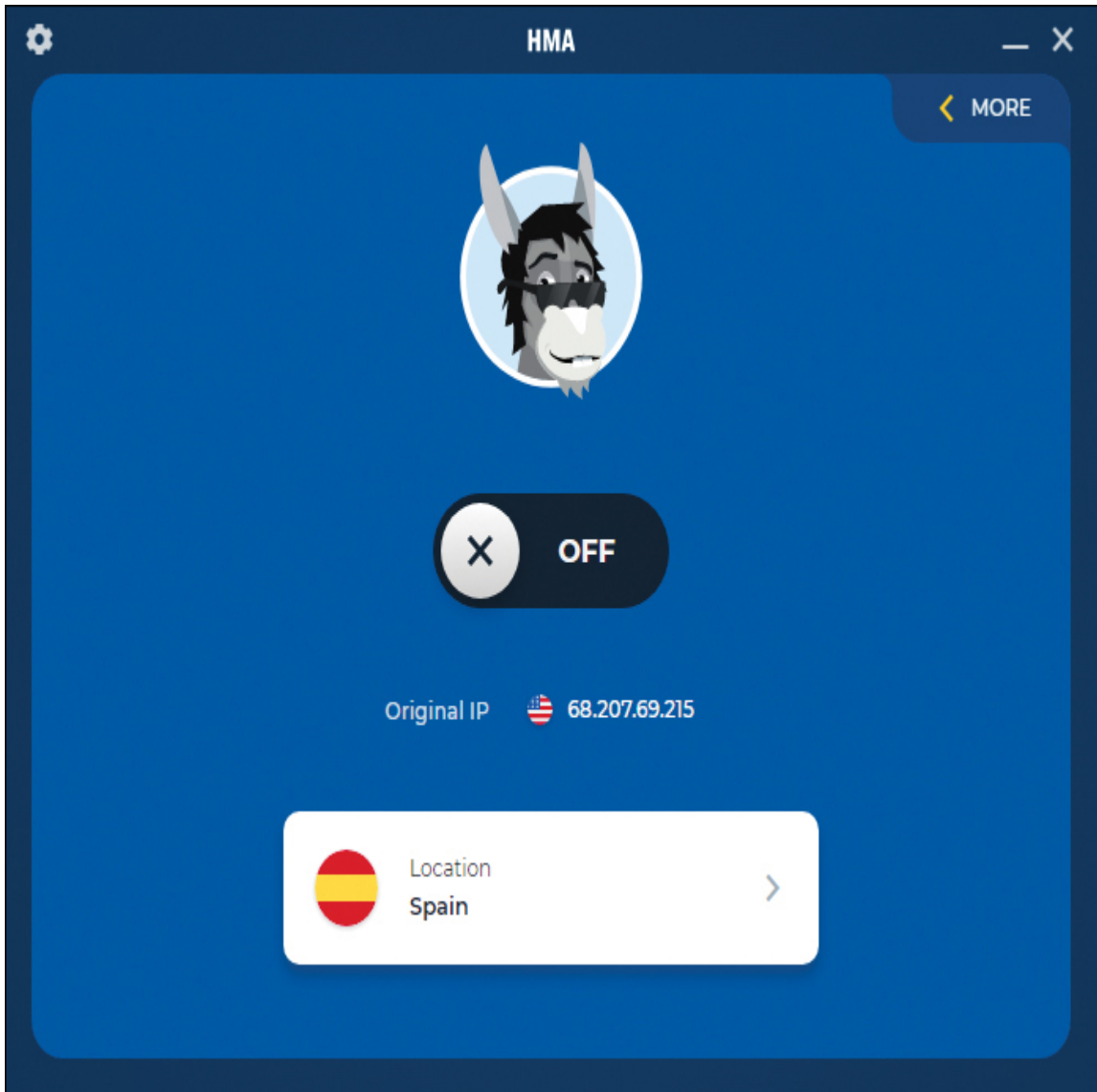
Figure 3.6 HMA.
