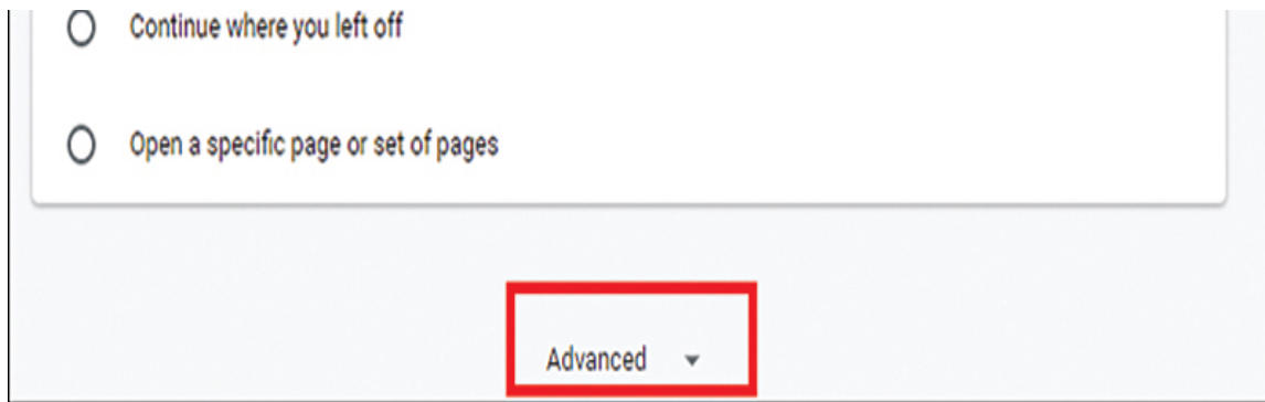
Figure 3.5 Chrome settings.
