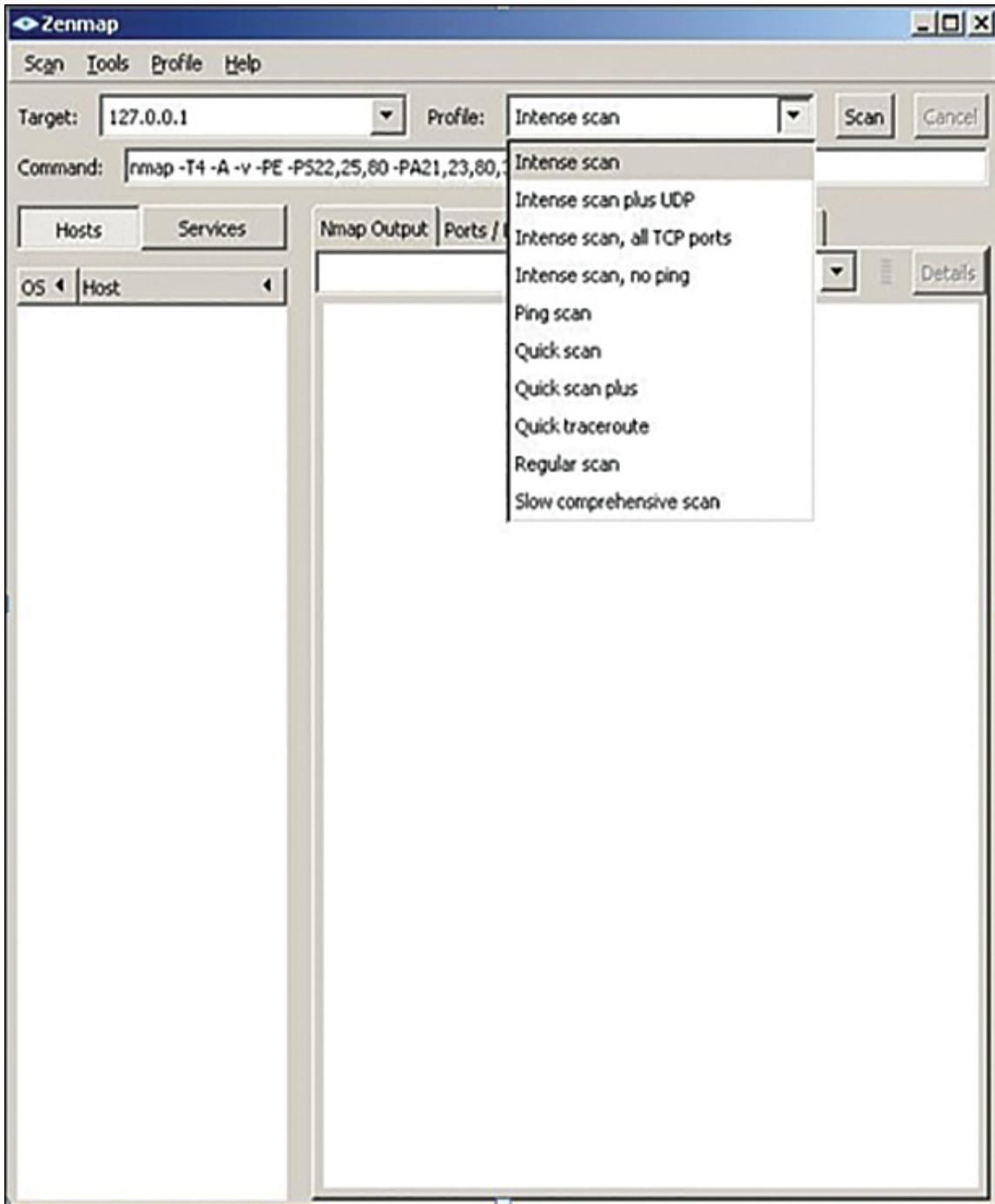
Figure 6.3 Zenmap GUI.
