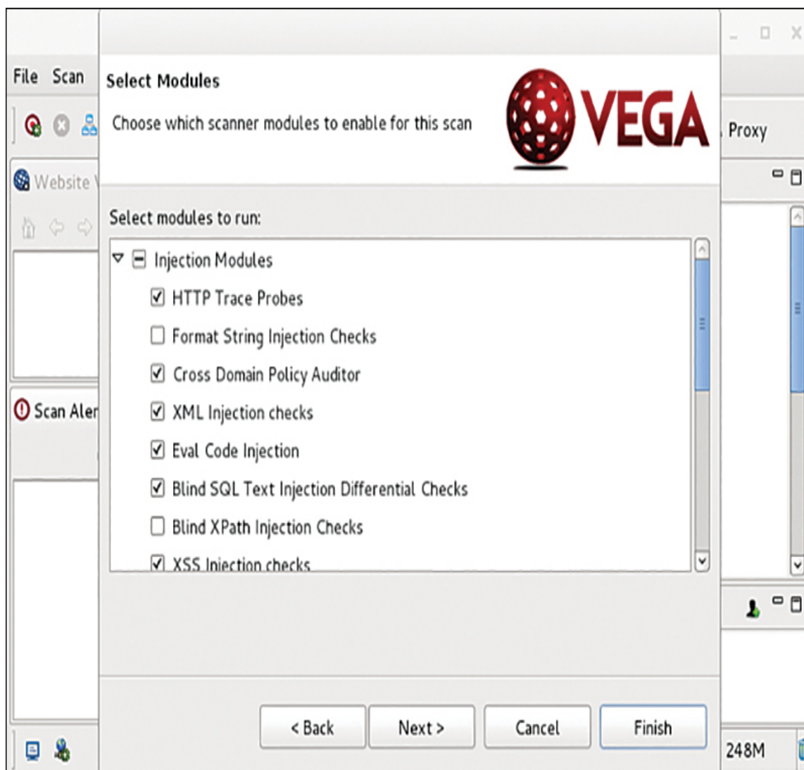
Figure 11.18 Vega scan.
