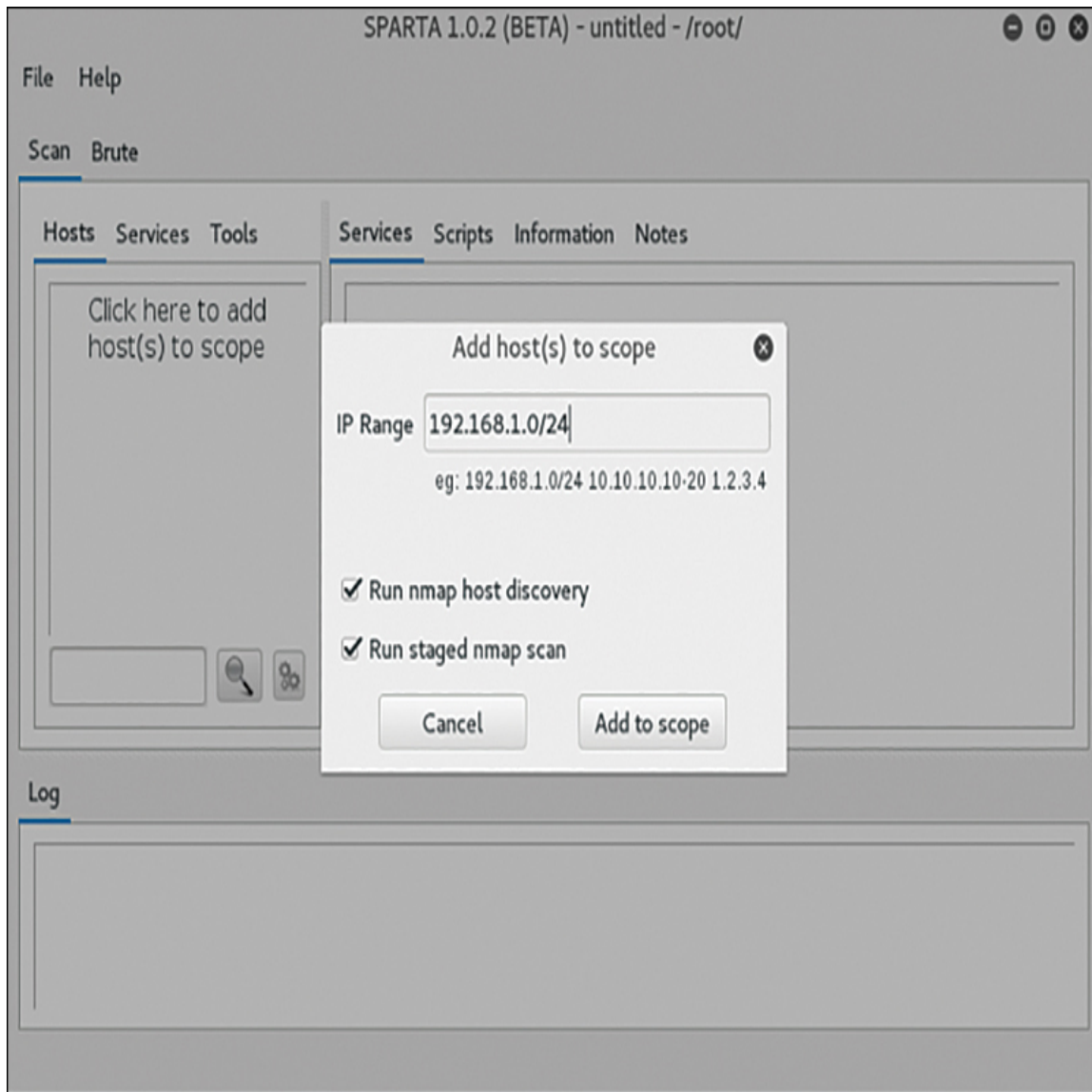
Figure 11.16 Sparta step 2.
