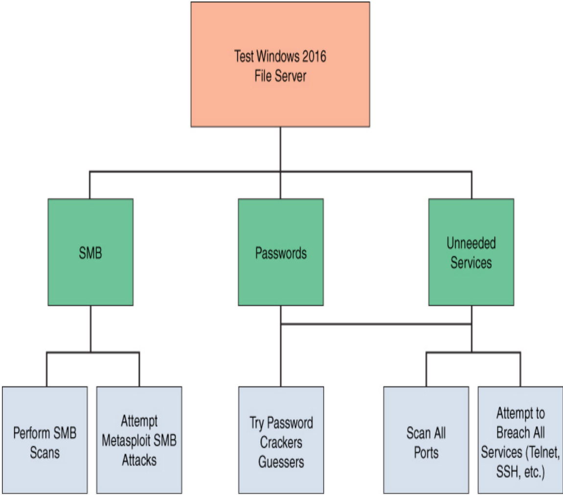
Figure 15.2 Work Breakdown Structure.
