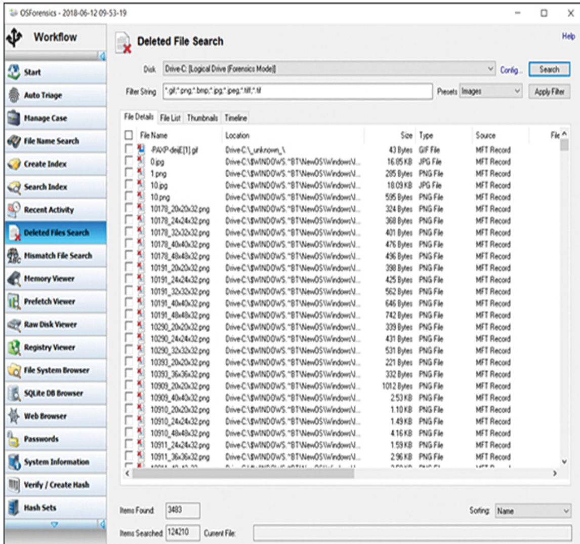
Figure 14.11 OSForensics Deleted File Search Option.
