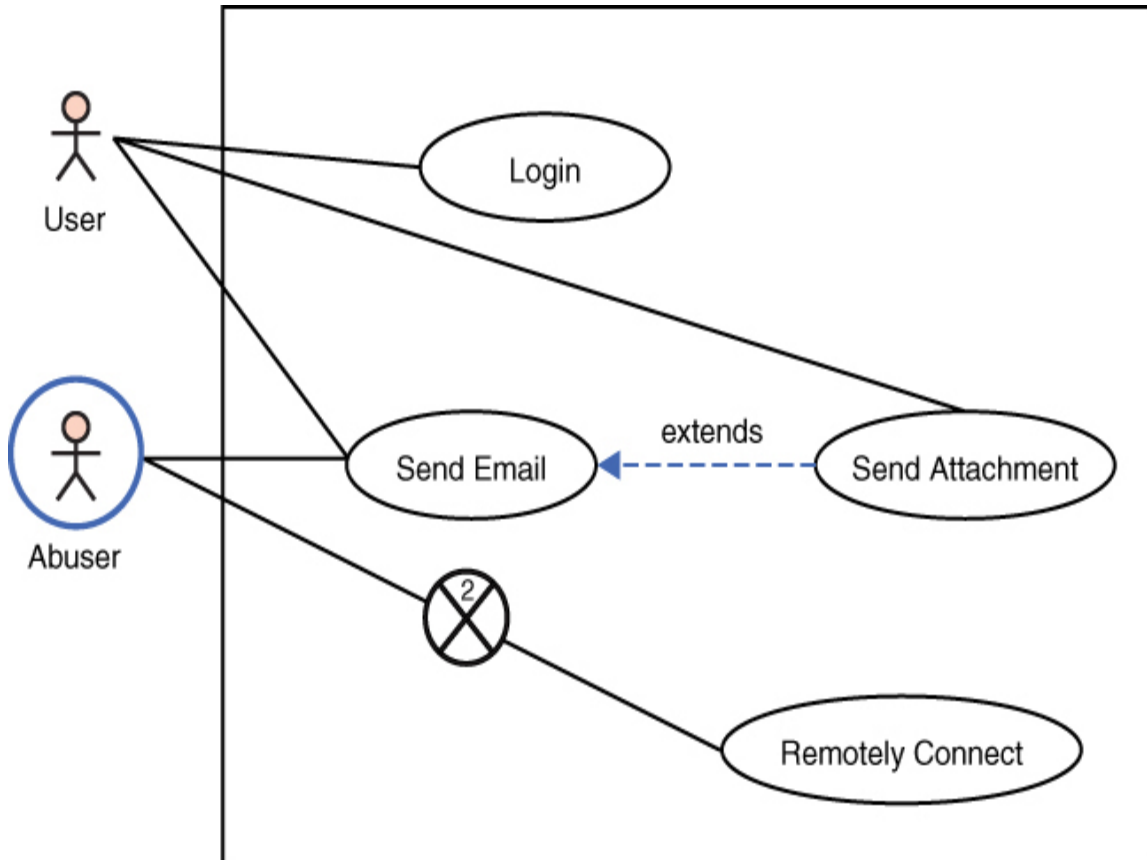
Figure 15.11 Specific misuse-case example.
