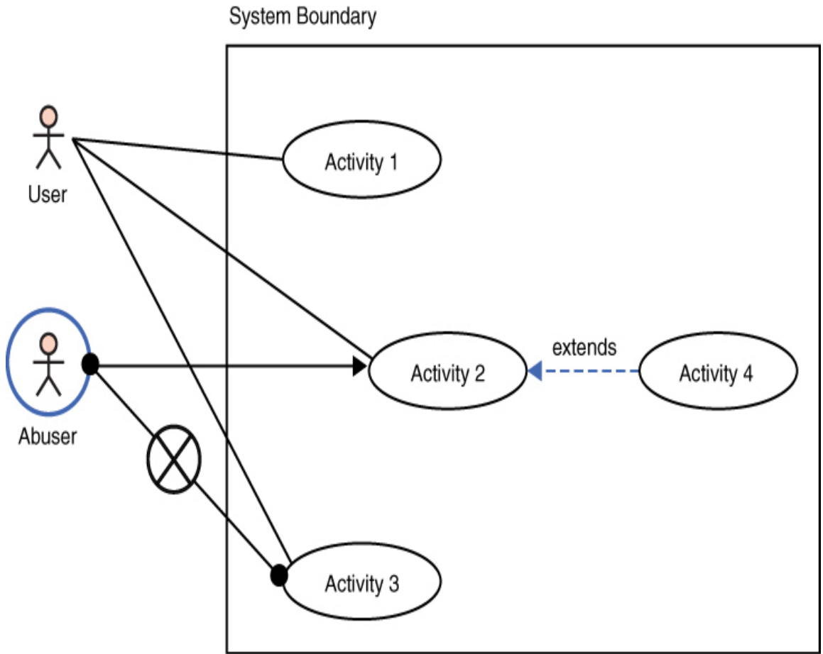
Figure 15.9 Misuse-case diagram example.
