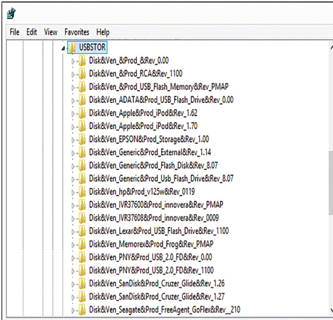
Figure 14.17 Windows Registry—USBSTOR.
