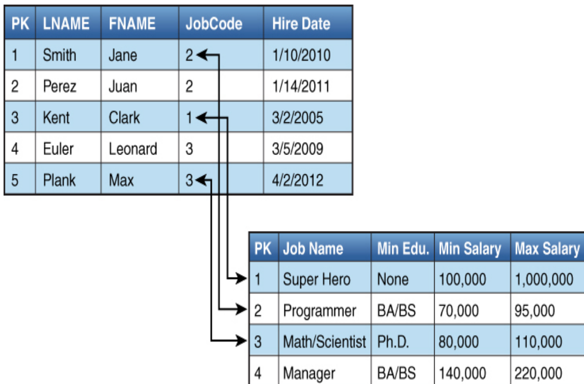
Figure 6.7 Database relations.
