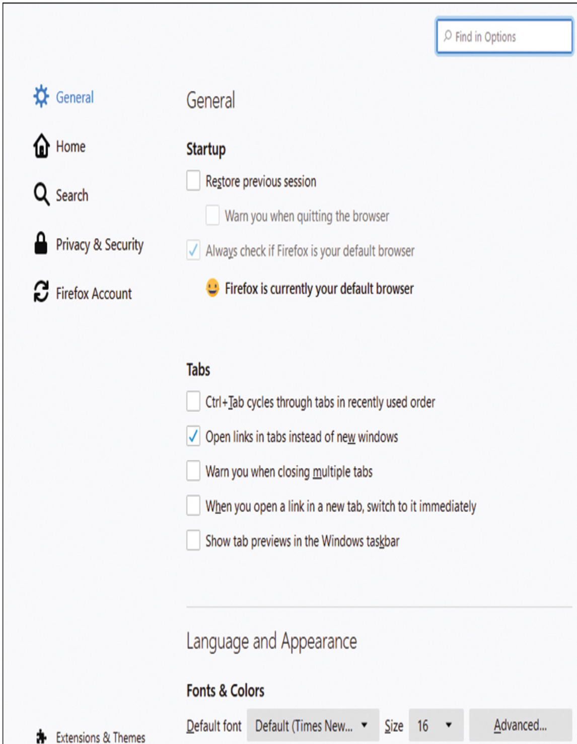
Figure 3.3 Firefox options.
