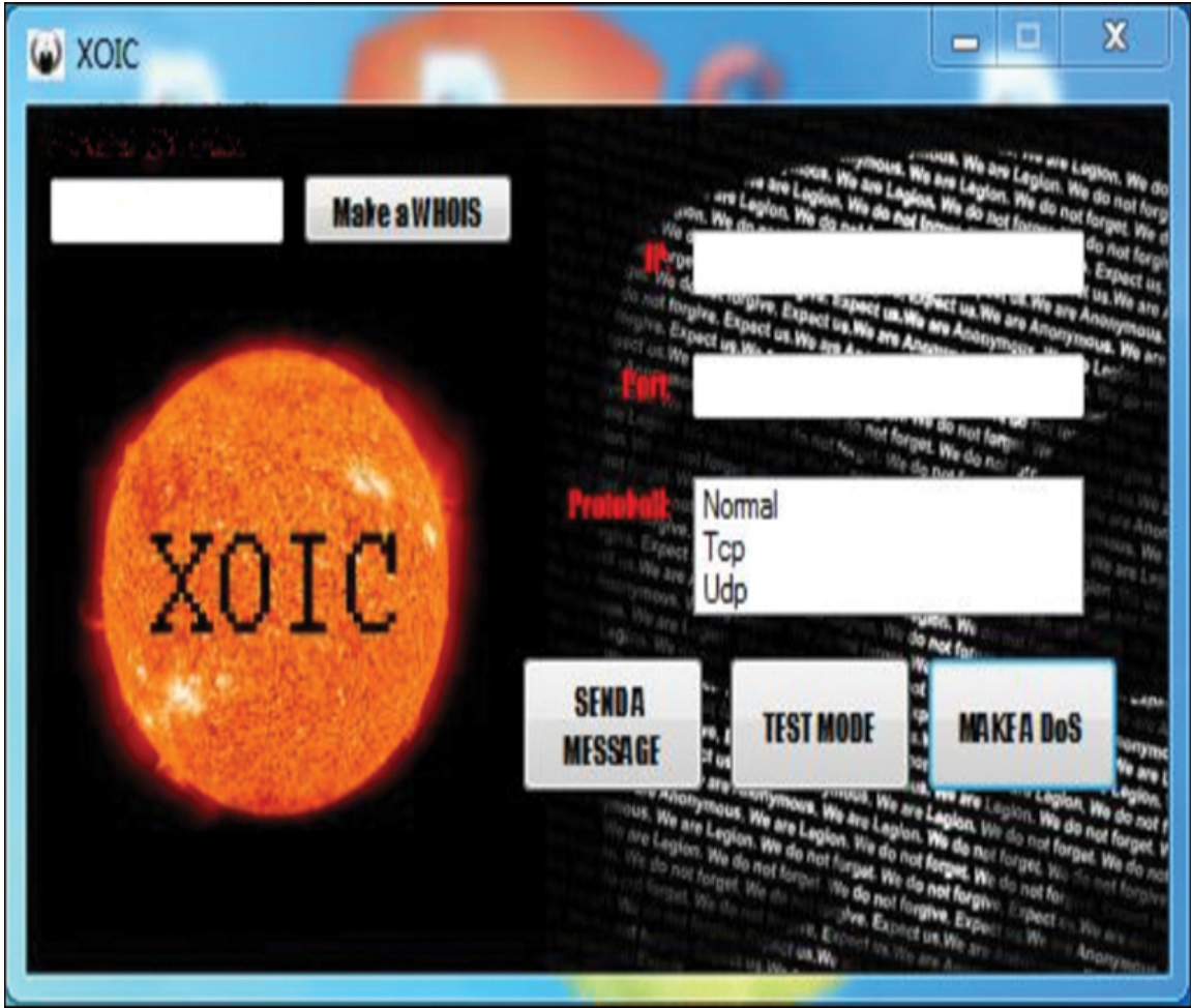
Figure 4.3 XOIC.
