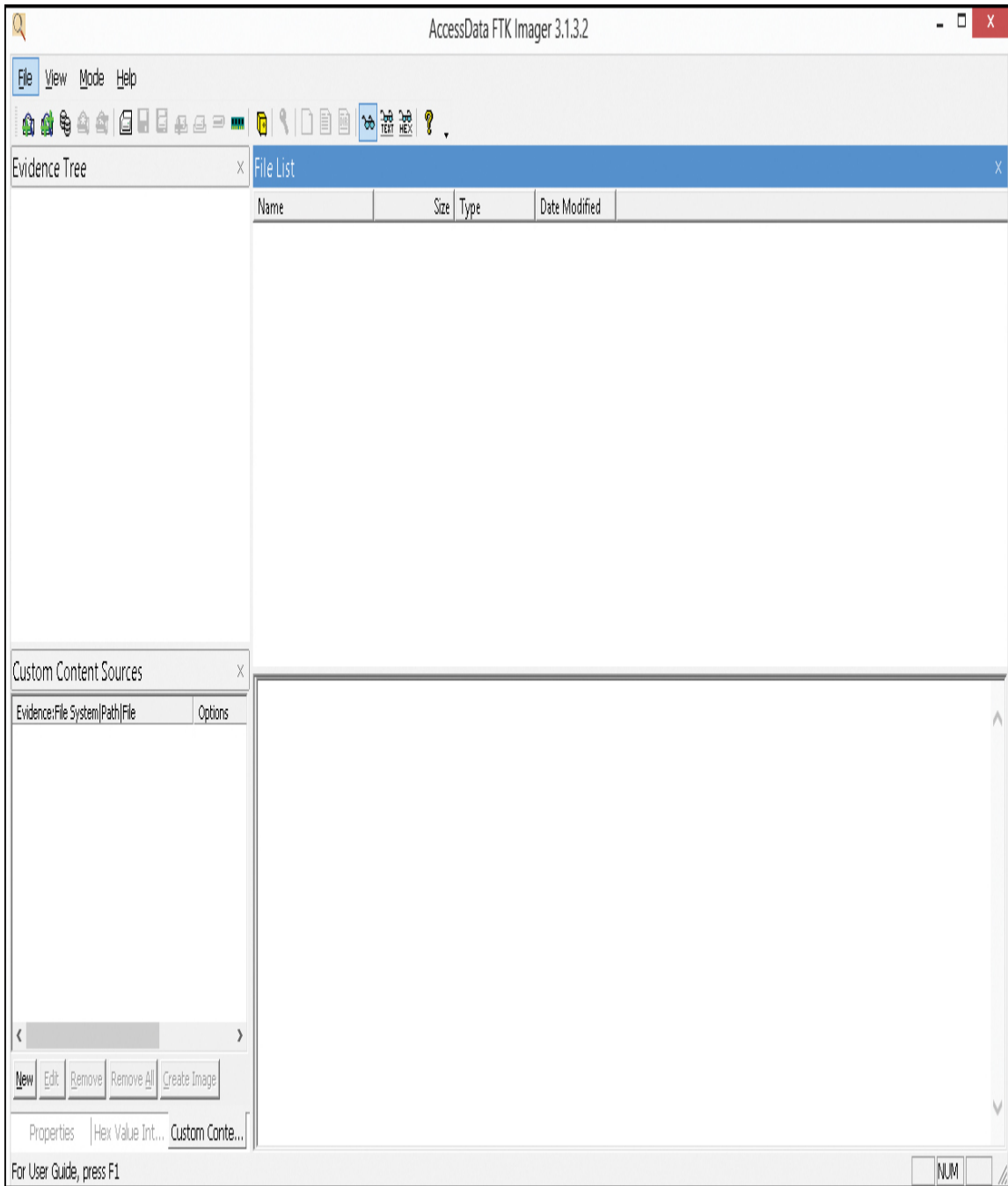
Figure 14.1 FTK Imager.
