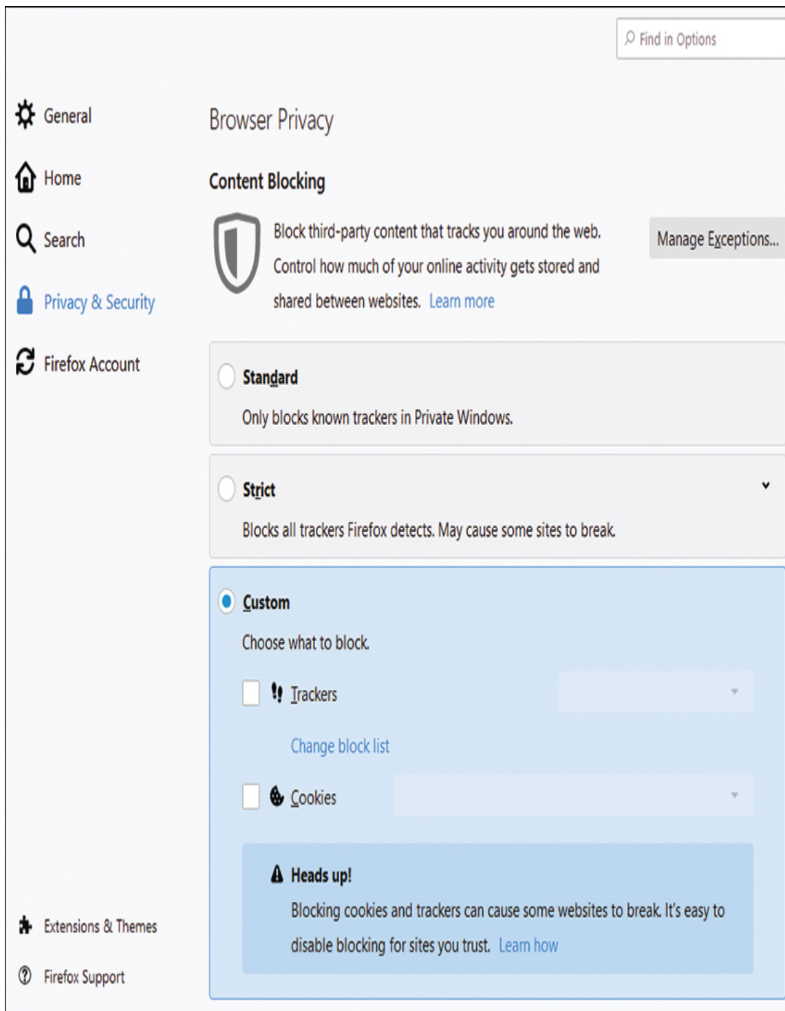
Figure 3.4 Firefox privacy.
