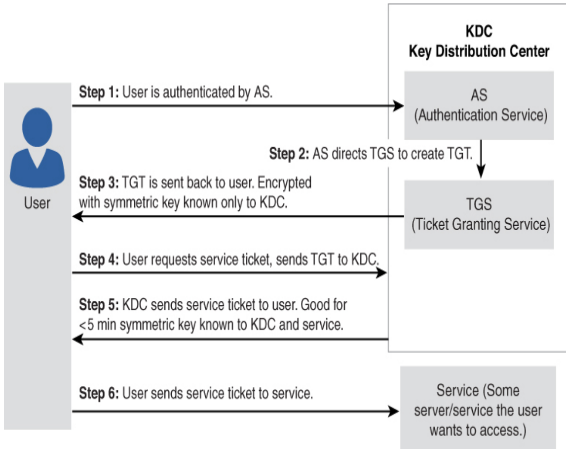
Figure 9.9 Kerberos.
