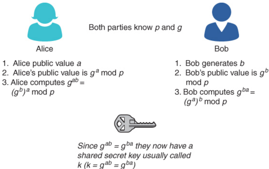
Figure 8.7 Diffie-Hellman.
