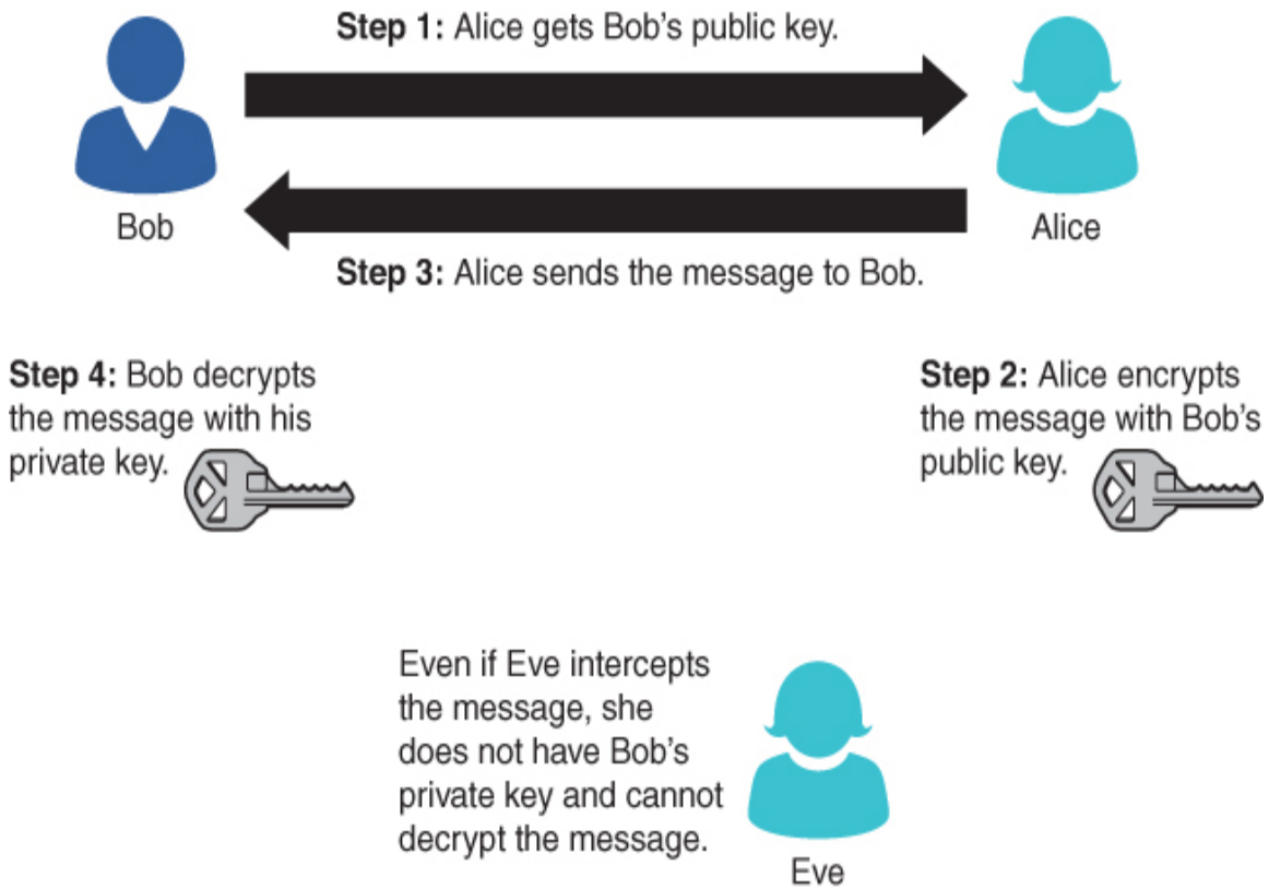
Figure 8.6 Public key cryptography.
