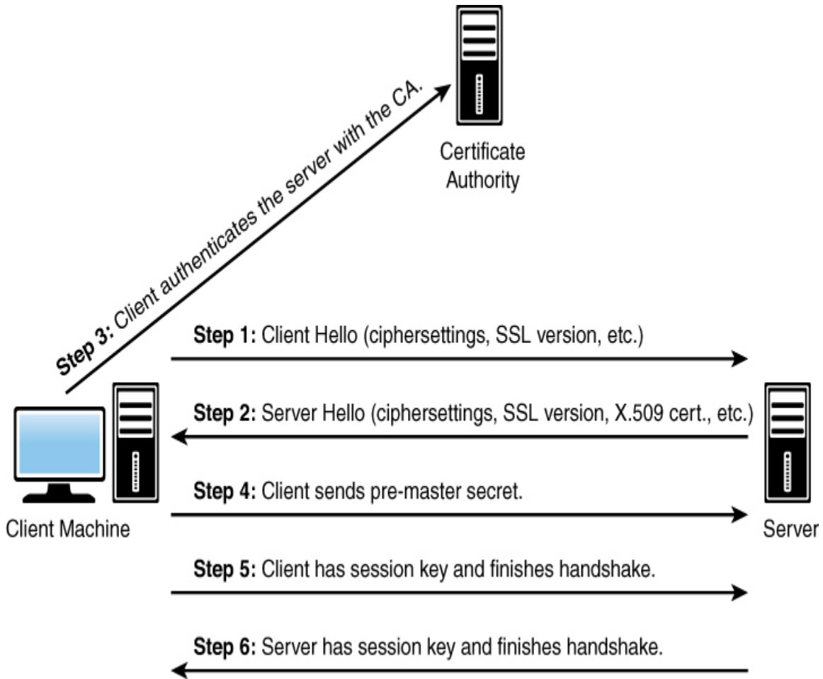
Figure 9.10 SSL/TLS.
