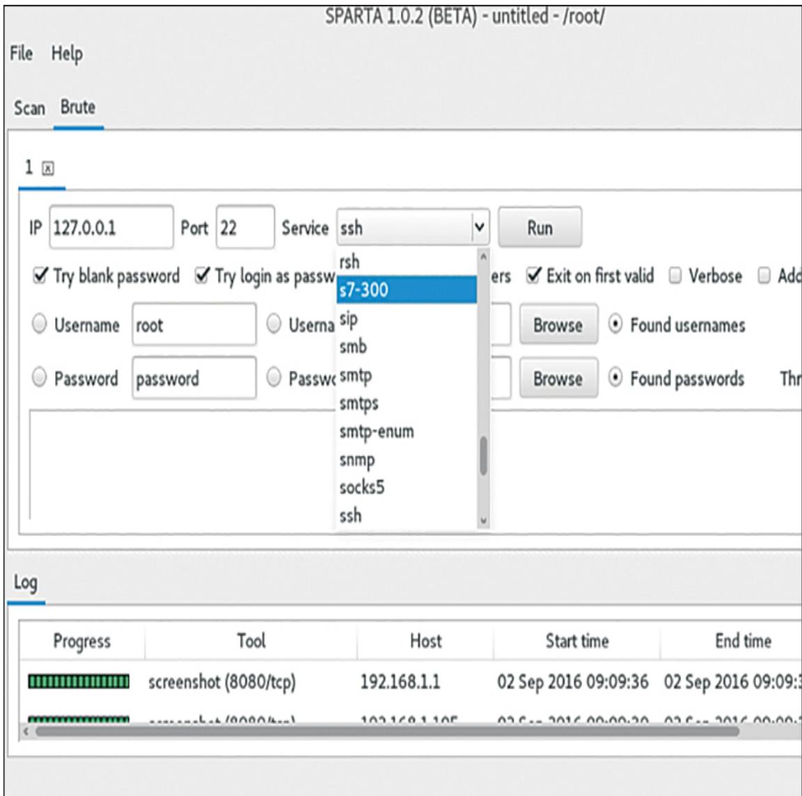
Figure 11.17 Sparta step 3.
