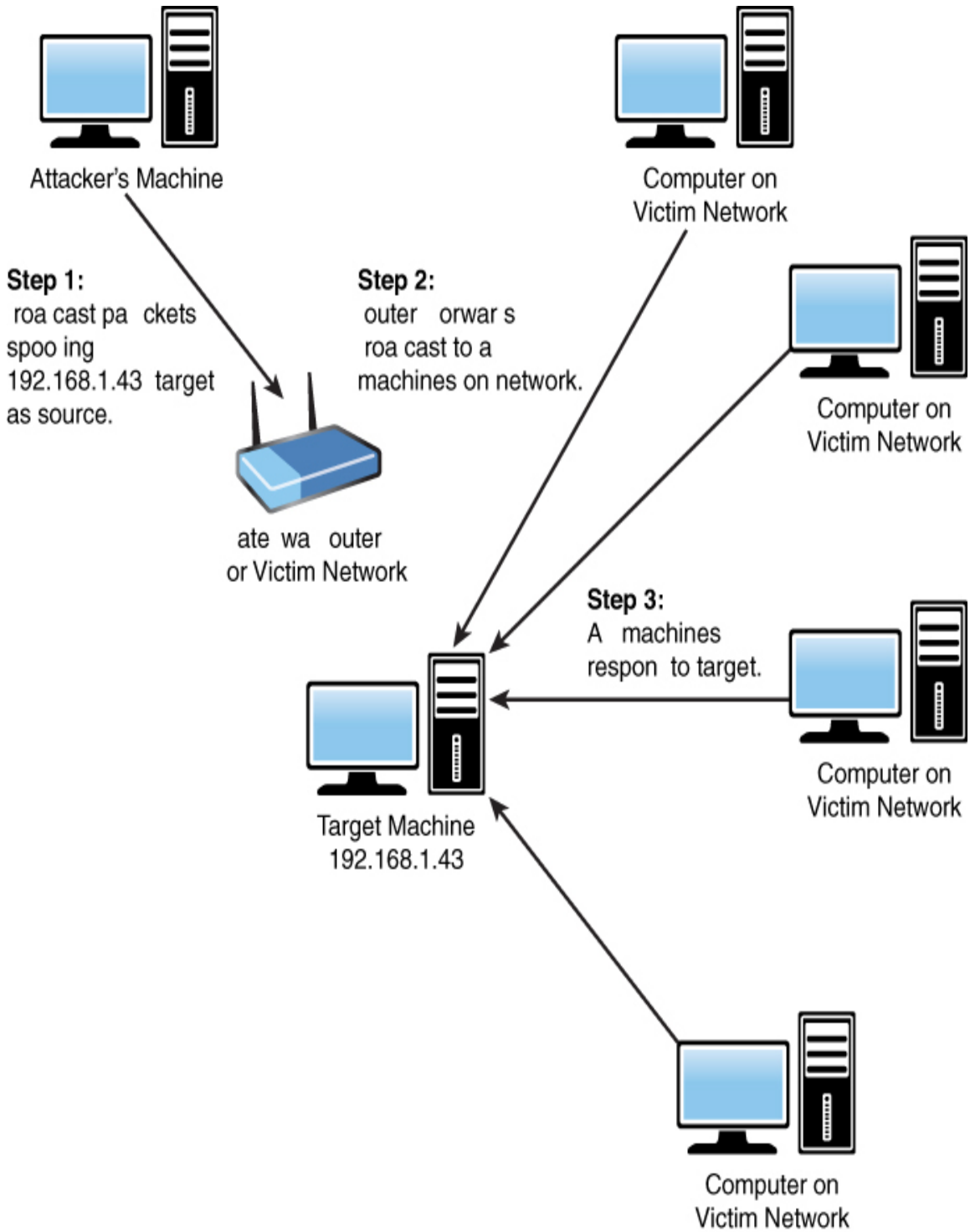
Figure 4.4 Smurf attack.
