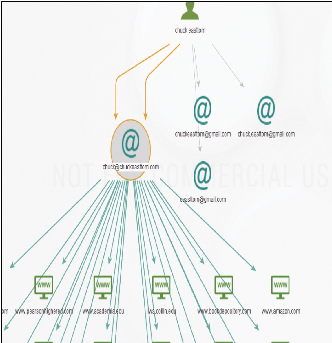
Figure 13.10 Maltego graph.
