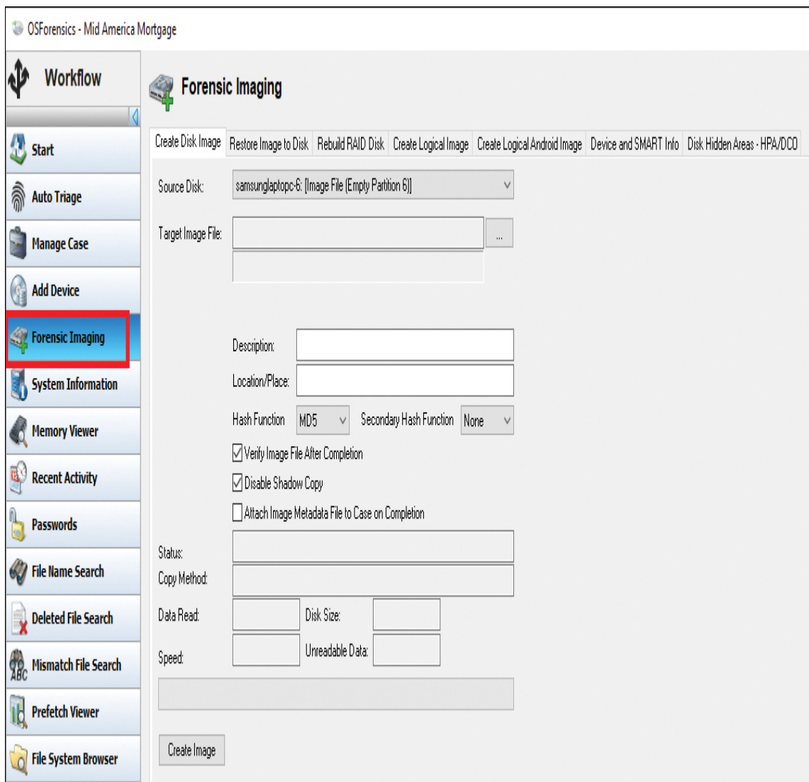
Figure 14.6 OSForensics Imaging.
