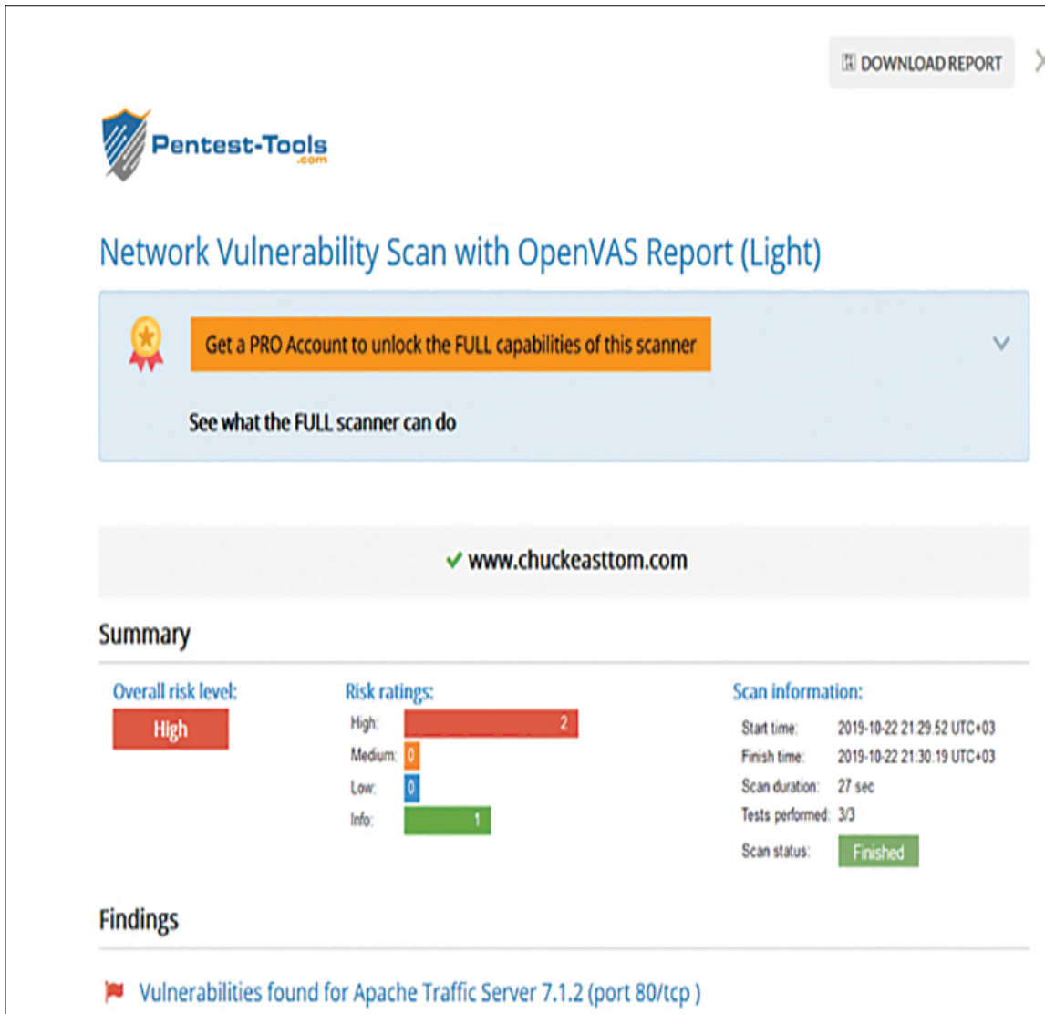
Figure 11.19 OpenVAS results.
