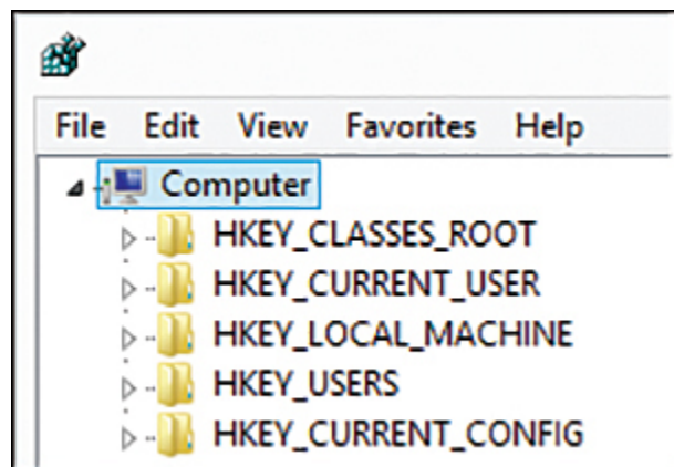
Figure 14.16 Windows Registry.
