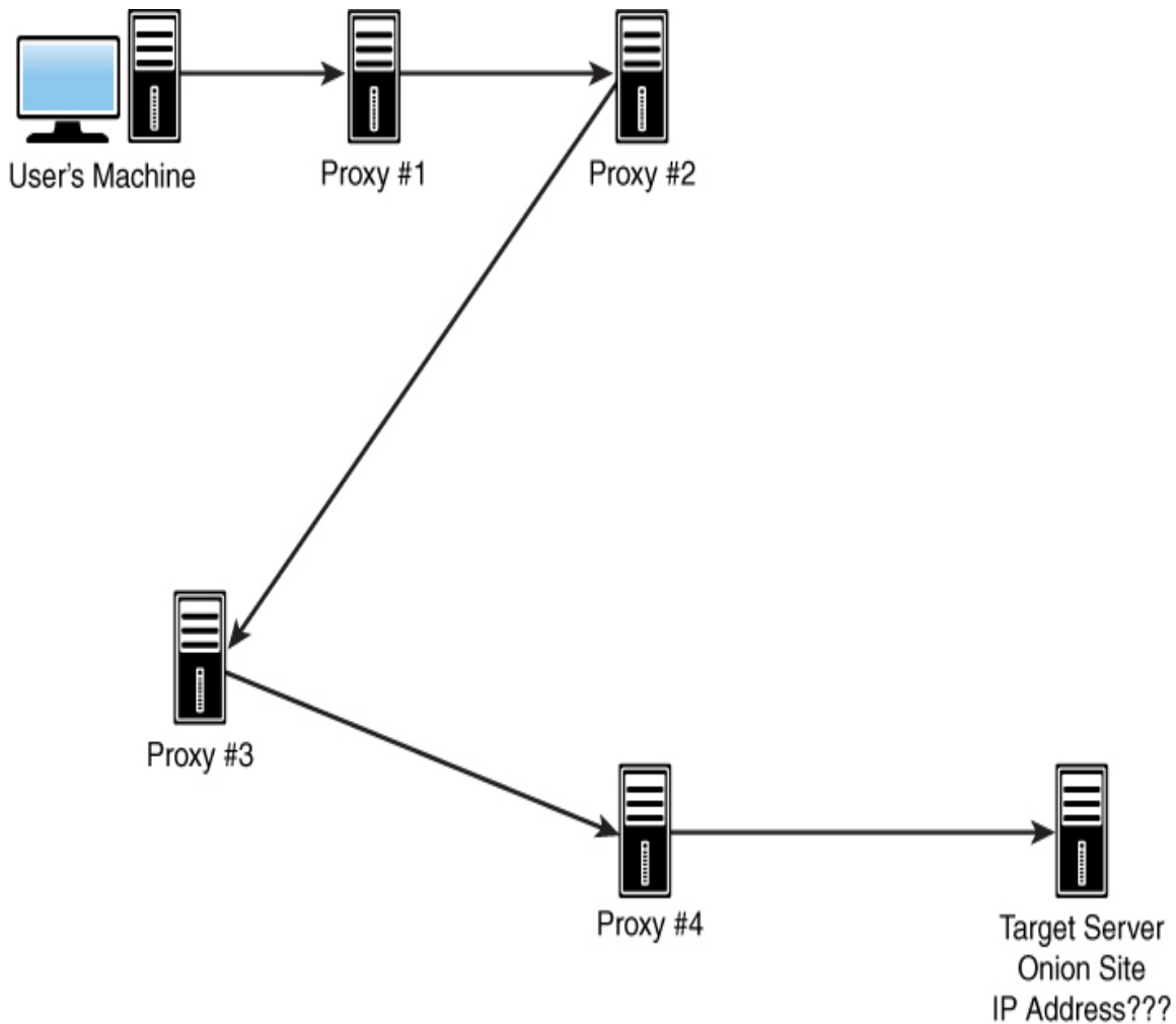
Figure 6.10 TOR.
