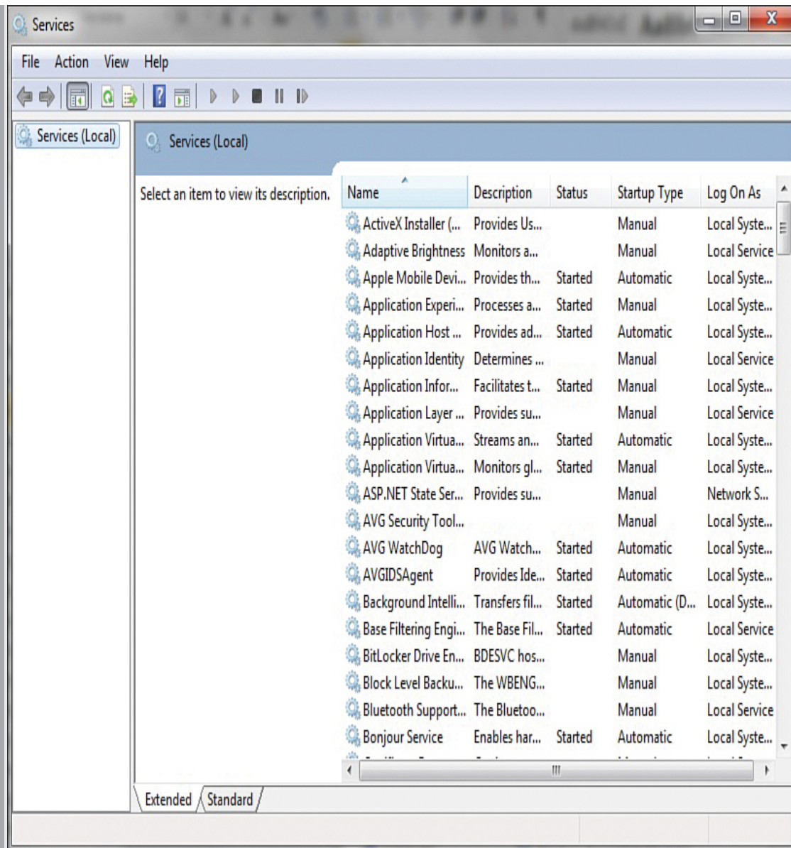
Figure 11.1 Windows services.
