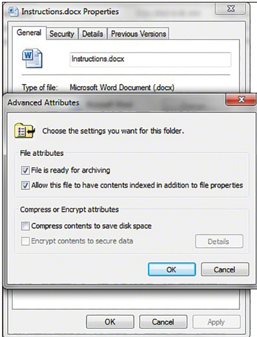
Figure 7.6 Windows EFS.
