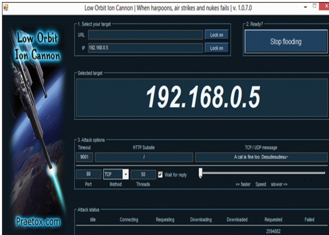
Figure 4.2 LOIC.
