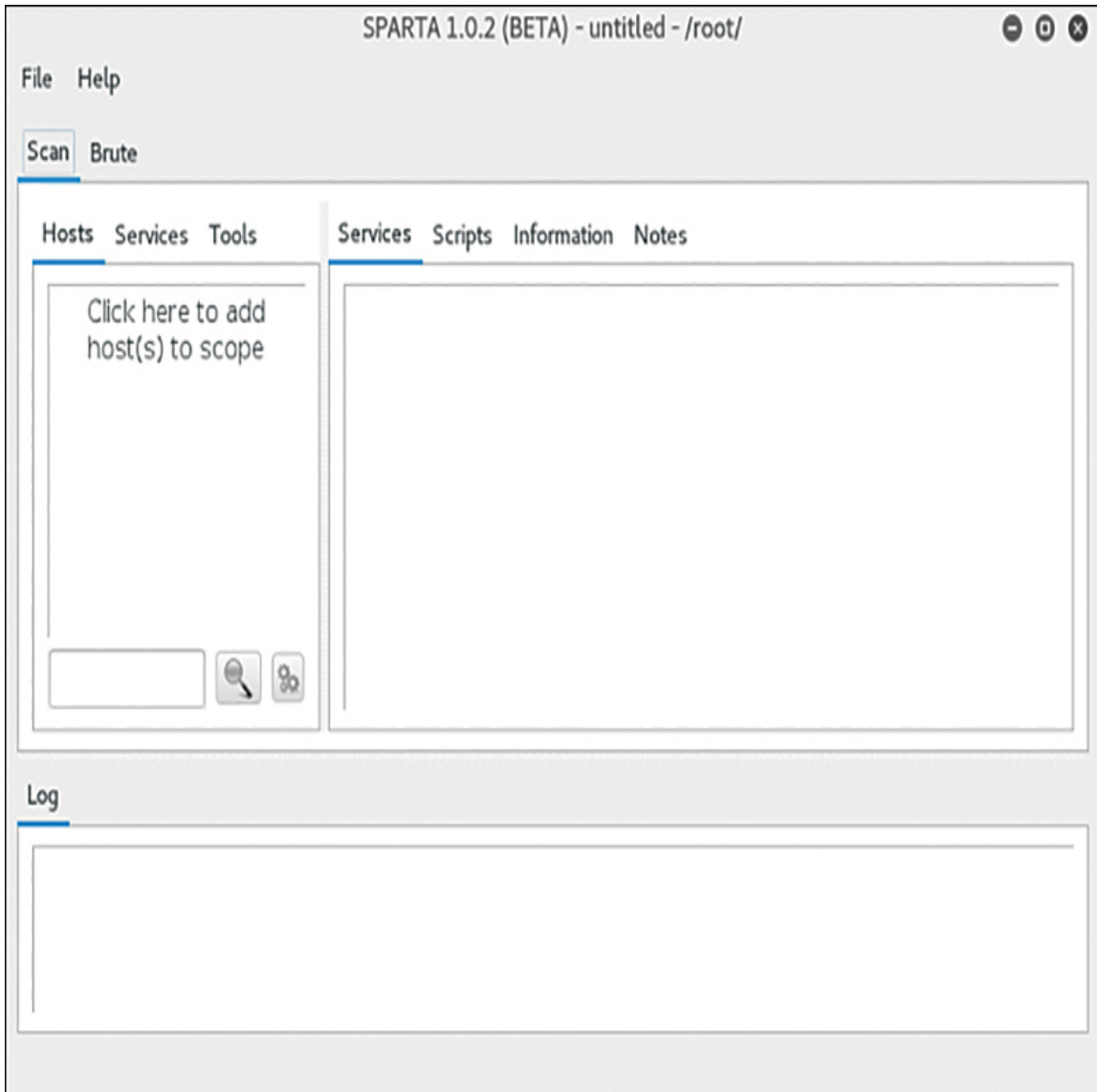
Figure 11.15 Sparta step 1.
