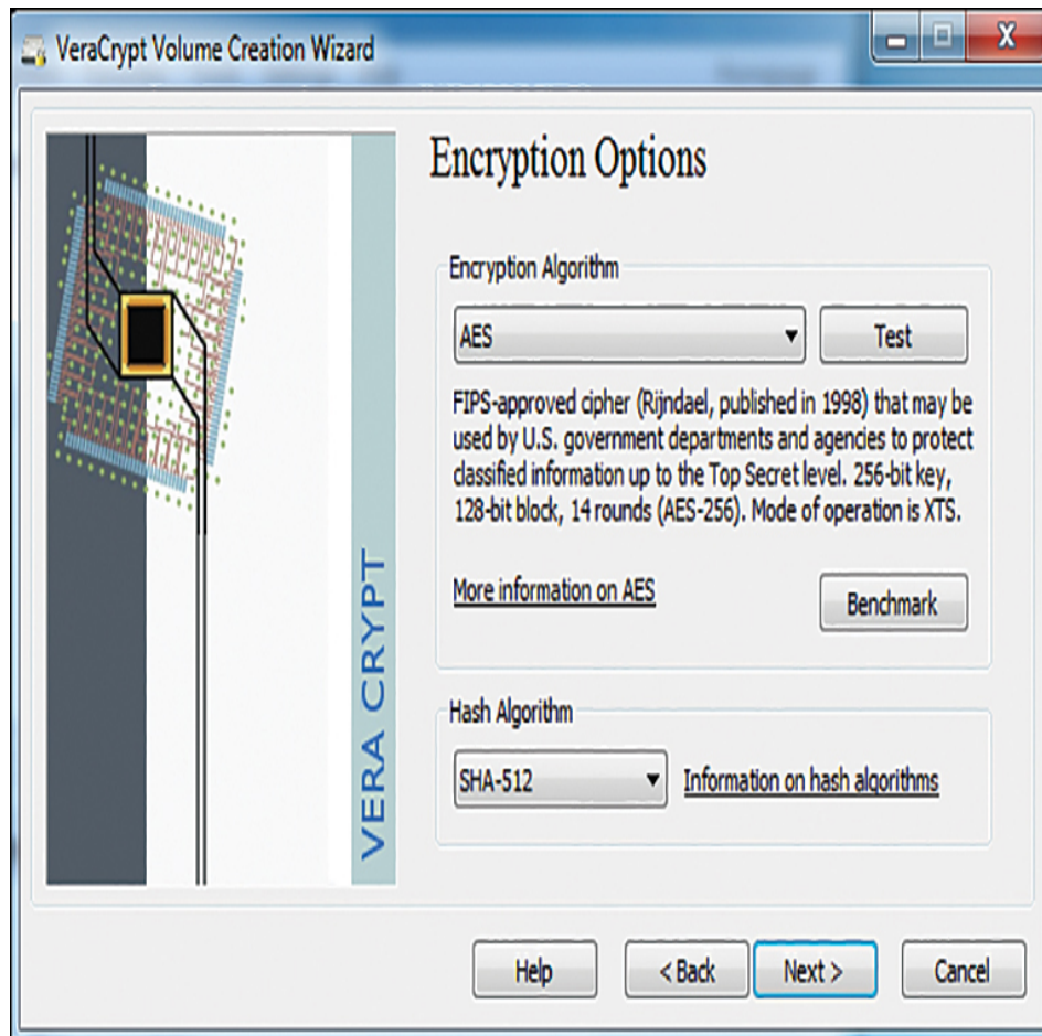
Figure 7.5 VeraCrypt.
