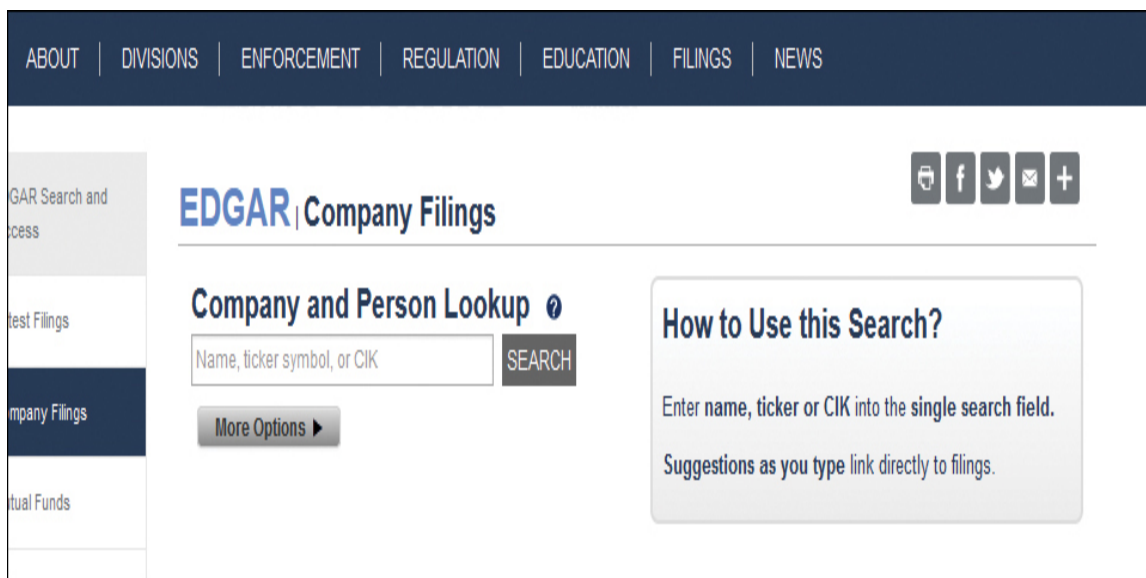
Figure 13.4 SEC search.
