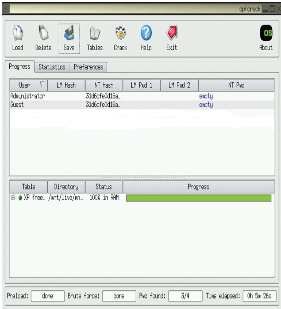
Figure 6.8 ophcrack.
