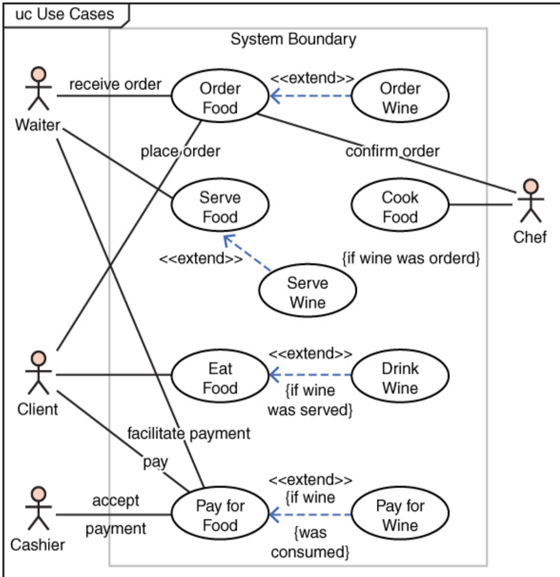
Figure 15.7 Typical use-case diagram.
